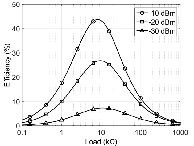
Fig. 5. Simulated rectifier efficiency versus load for different power input levels at 868 MHz.
