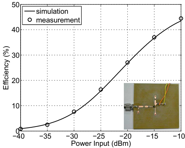
Fig. 3. Simulated and measured rectifier efficiency versus power input at 868 MHz.
